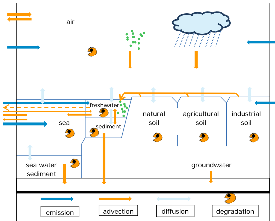
Figure R.16-6: Schematic representation of the model for calculating the regional PECs
